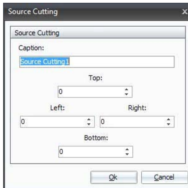
Figure 10.5: Source Cutting
