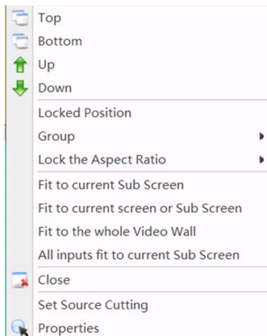
Figure 10.4: Zooming
